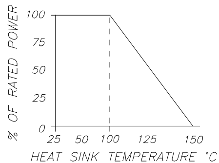
DERATING CURVE:
