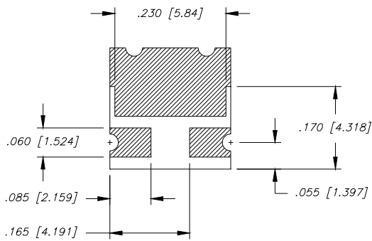
Dimensions in inches Tolerance \pm .010 unless otherwise stated
