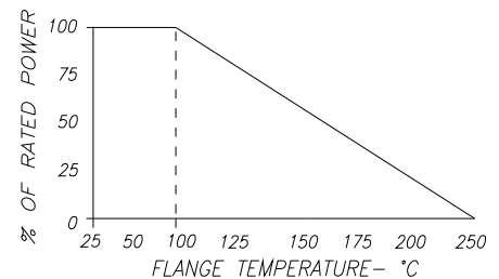
DERATING CURVE:
