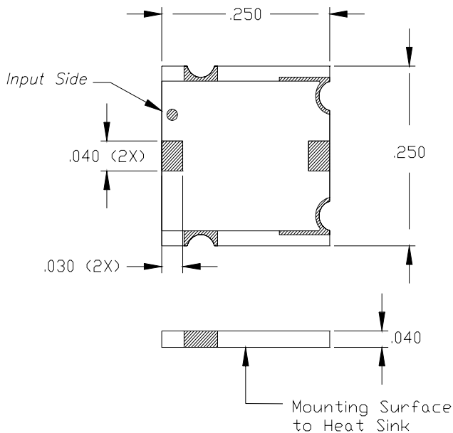
Dimensions in inches Tolerance ± .010 unless otherwise stated
