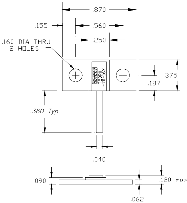
Dimensions in inches Tolerance ± .010 unless otherwise stated
