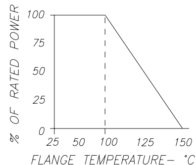
DERATING CURVE:
