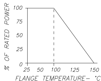
DERATING CURVE:
