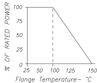
DERATING CURVE:
