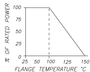
DERATING CURVE:
