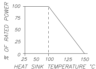
DERATING CURVE:
