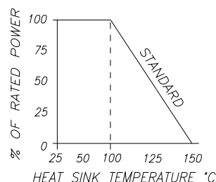
DERATING CURVE:
