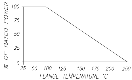
DERATING CURVE:
