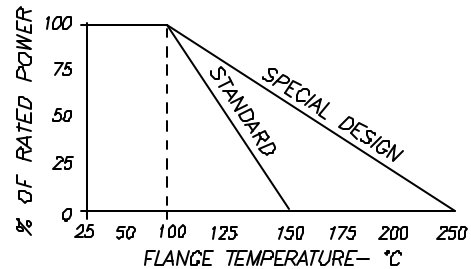
DERATING CURVE:
