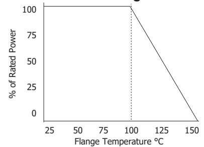
TA50R0-100-24X Power Derating Curve
