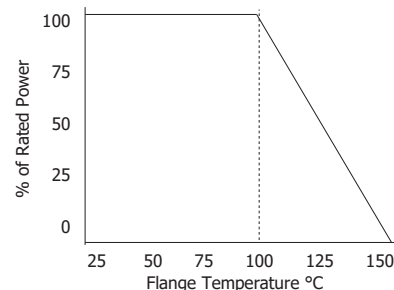
T50R0-40-17X Power Derating Curve
