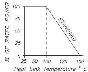
DERATING CURVE:
