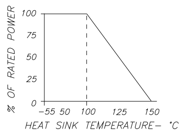
DERATING CURVE:
