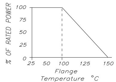
DERATING CURVE:
