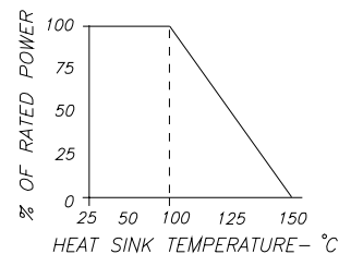
DERATING CURVE:
