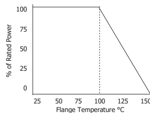
A1100-100-11X Power Derating Curve
