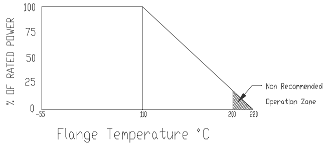
DERATING CURVE
