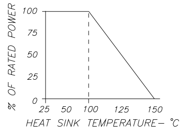
DERATING CURVE:
