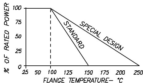
DERATING CURVE:
