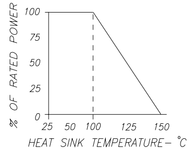
DERATING CURVE:
