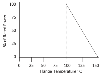
AA1000-250-17X Power Derating Curve
